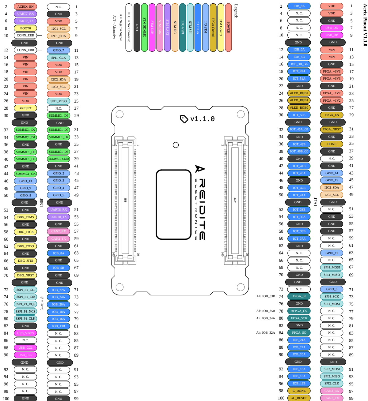
Figure 1: Pinout diagram with color-coded legend.
